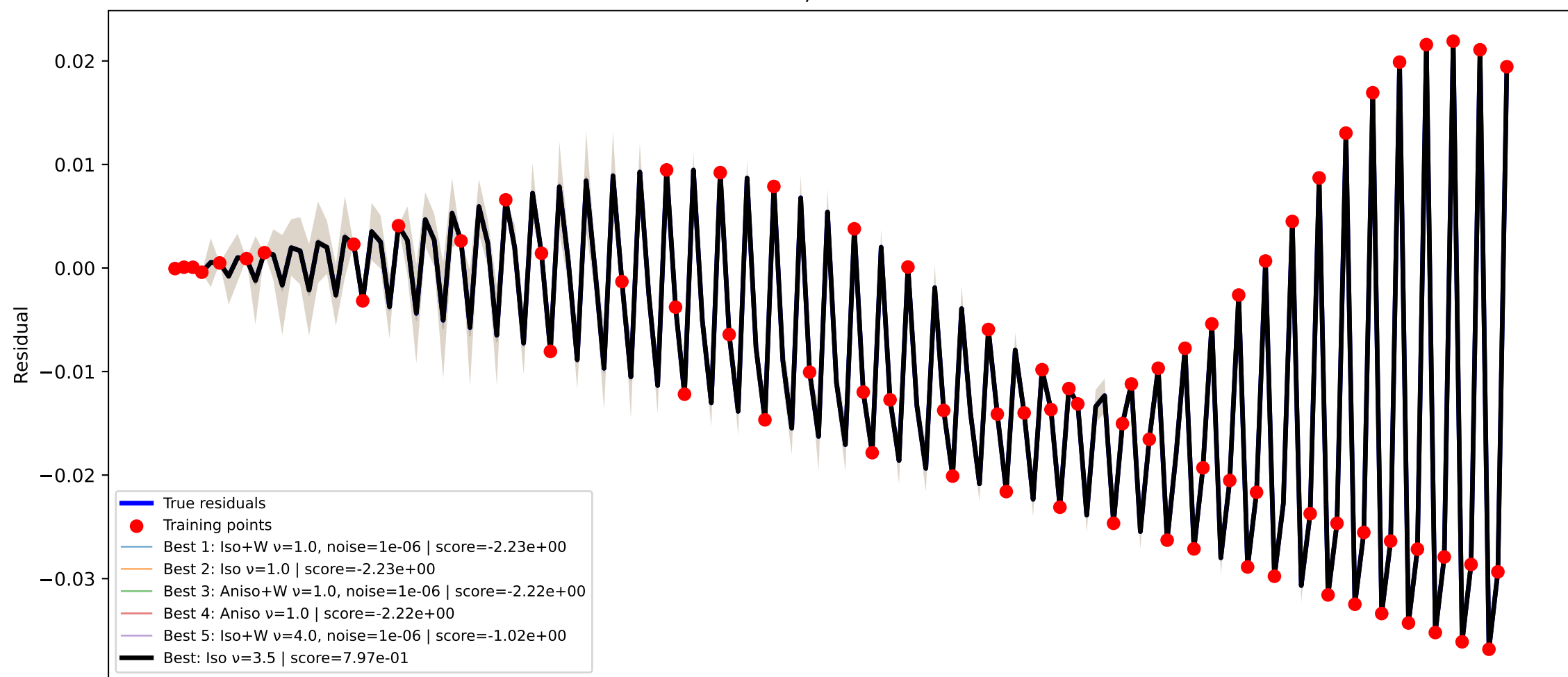
GPR kernel comparison node=6 RMSE=6.768e-06, train RMSE=3.892e-09
